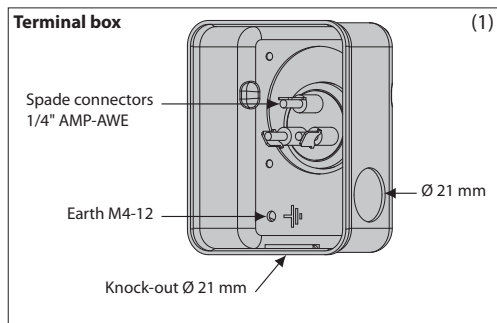
IP rating: 55 (with cable gland)
