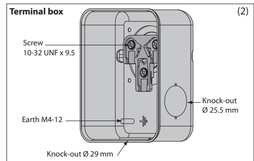
IP rating: 54 (with cable gland)
